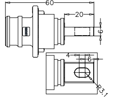
ES8 MALE CONNECTOR
