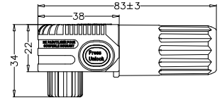
ES8 FEMALE 90° SHAPE CONNECTOR
