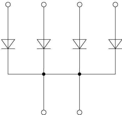
Circuit Diagram
